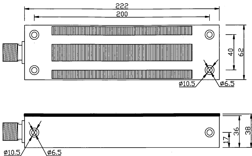
Magnetic lock dimension drawing
