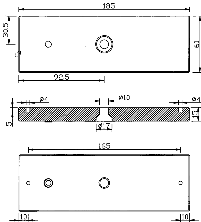
Adsorption board size chart
